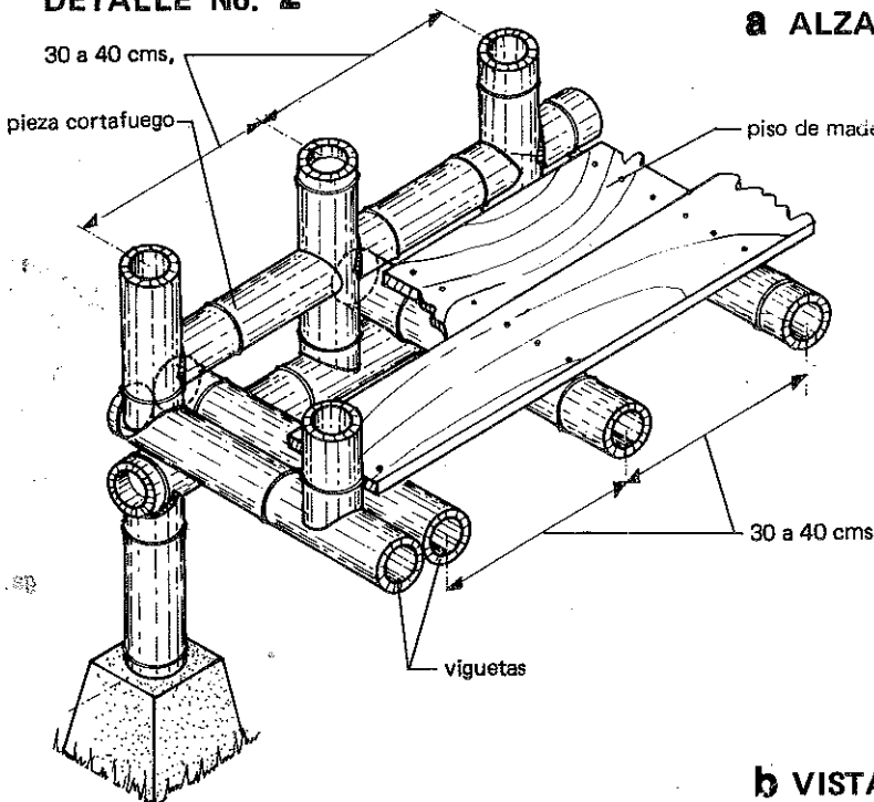
DETALLE No. 2
