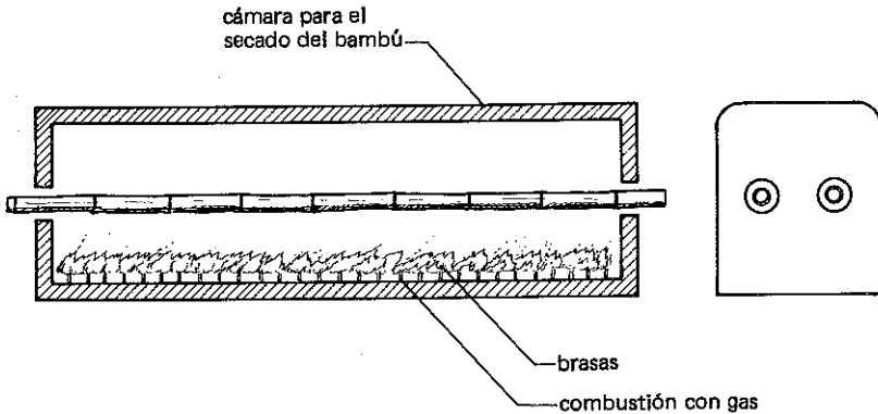
DETALLE No. 2
