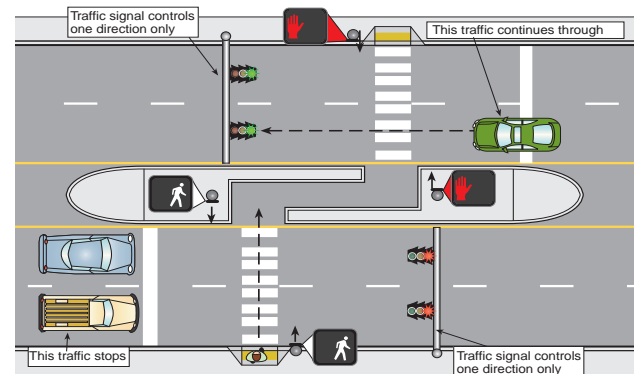
Figure 5-25: 2-step signal: pedestrian activates signal to stop near side traffic
