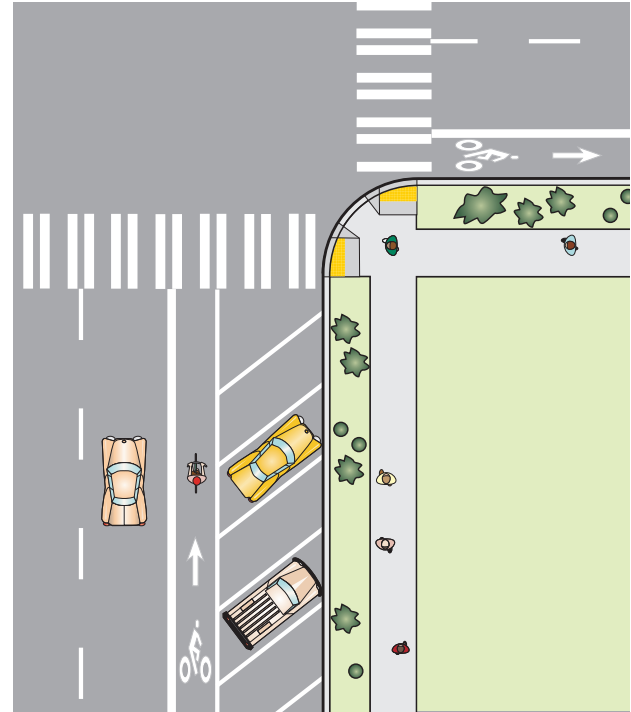
Figure 1-11: Bike lane next to diagonal parking
