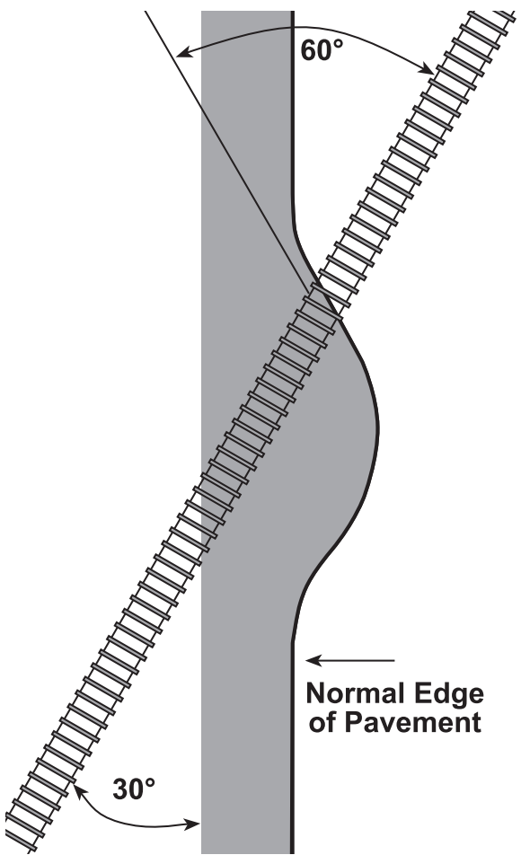
Figure 1-17: Bulged RR crossing
