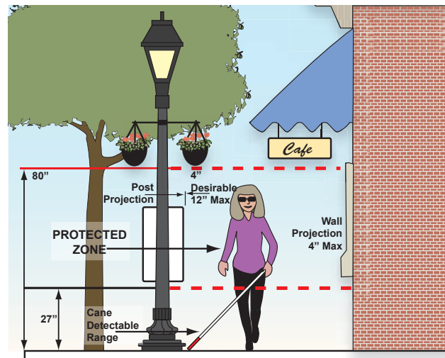
Figure 4-36: Blind pedestrian with clearances
