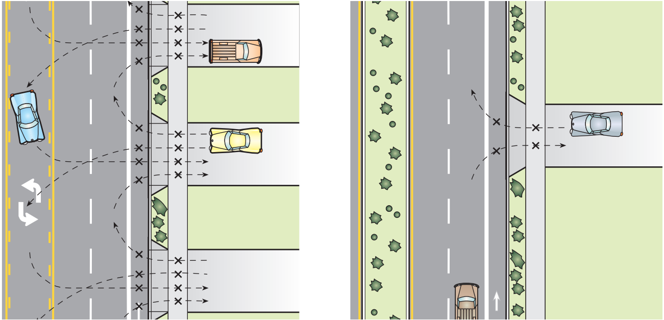
Figure 5-3: Access management techniques such as raised medians and consolidated driveways reduce conflict points
