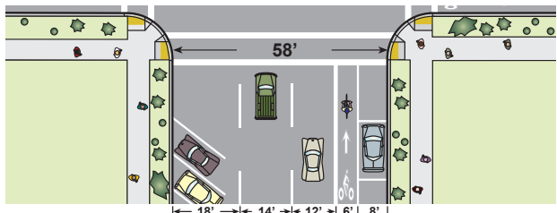
Figure 5-20: Crossing distance without curb extensions
