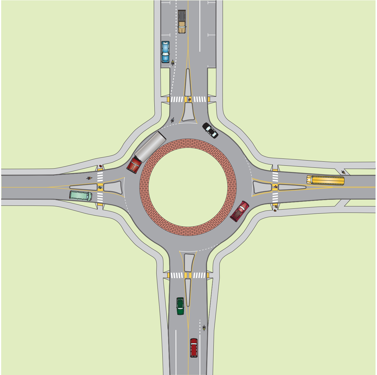
Figure 6-27: Modern roundabout
