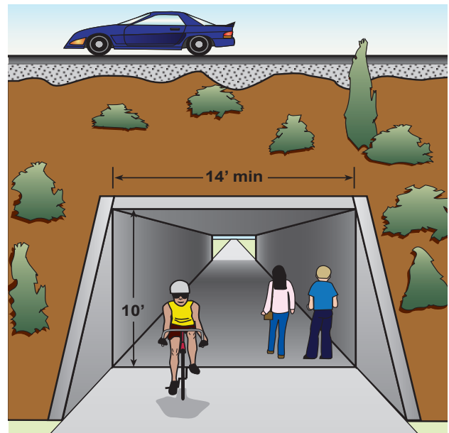
Figure 7-17: Undercrossing
