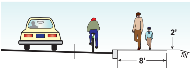
Figure 4-8: Recommended curb side sidewalk dimensions
