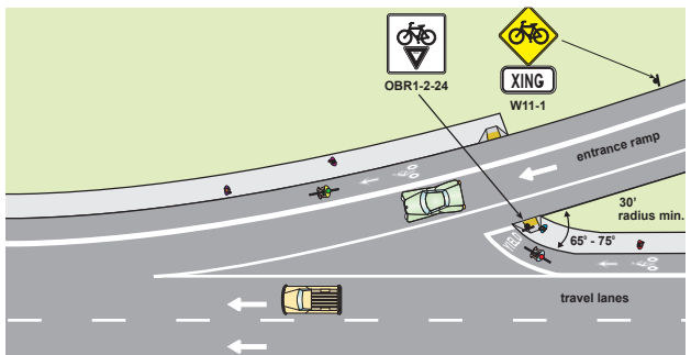
Figure 6-32: Bicyclist crossing at high speed entrance ramp
