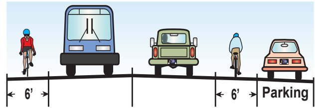
Figure 1-9: Typical bike lane dimensions
