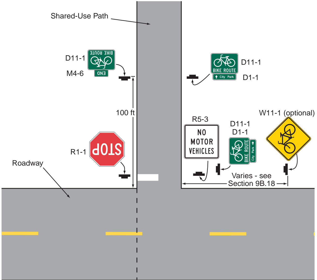
Figure 7-39: Beginning and end of path signing
