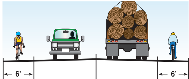
Figure 1-4: Shoulder bikeway
