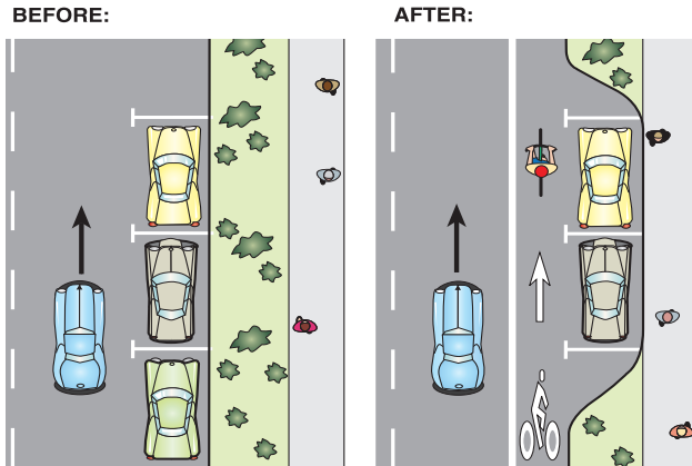
Figure 2-5: Parking bays
