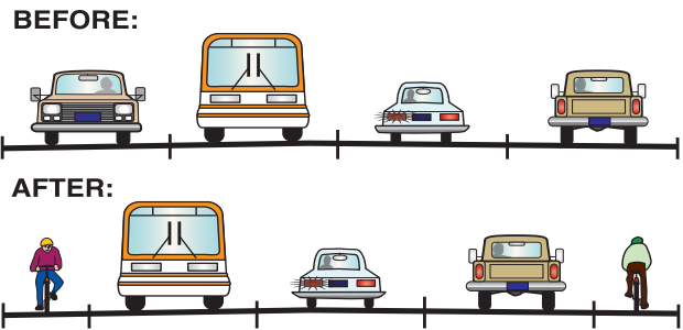
Figure 2-8: 4-lane, two way street restriped with 2 lanes in one direction, 1 in the other and bike lanes
