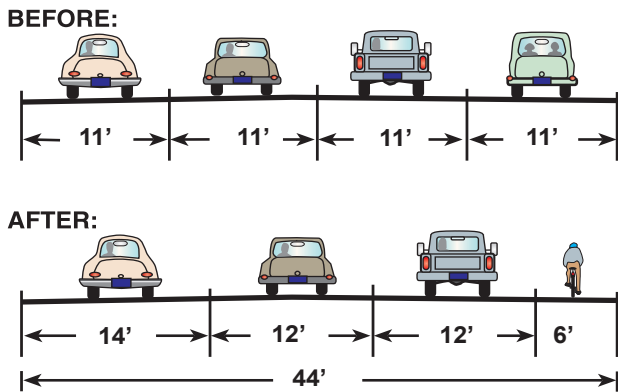
Figure 2-7: Motor vehicle travel lane removed from 4-lane, one way street
