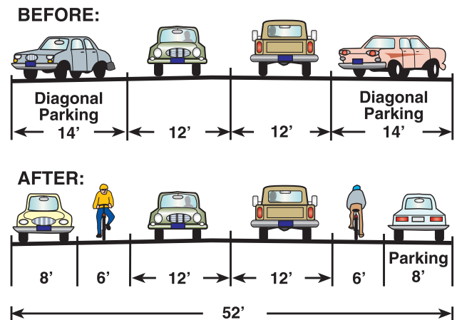
Figure 2-3: Restripe from diagonal to parallel parking
